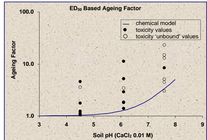
Figure 2: The ageing factors based on toxicity (symbols) and the predicted factor changes in isotopically exchangeable pool of Ni in soil (line). Open symbols are 'unbounded' values and are a lower estimate of the ageing factor
