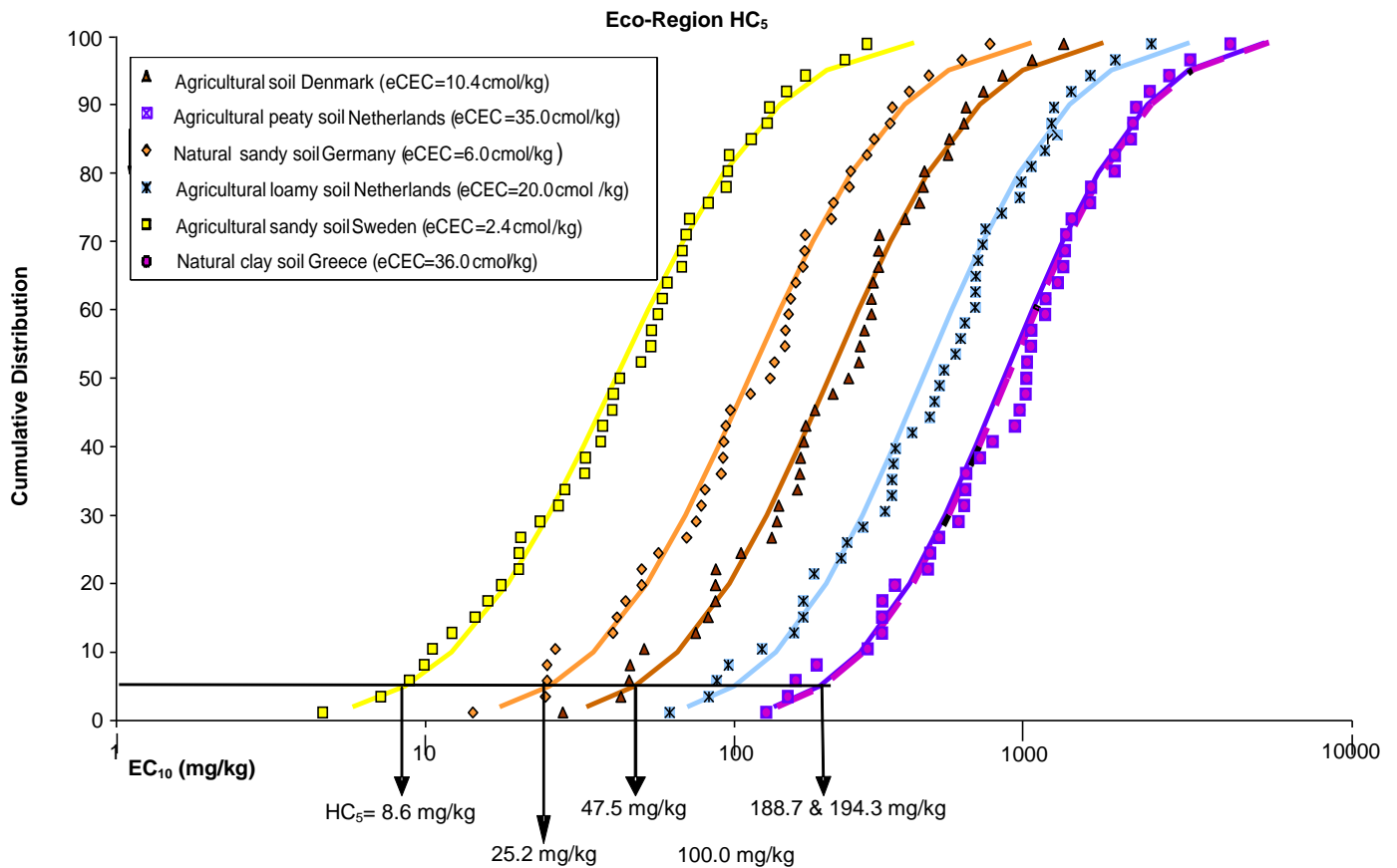
Figure 7: Overview of the SSD and HC 5 for the different selected soil eco-regions
